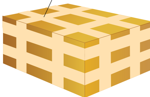
“井字棋”封箱法
