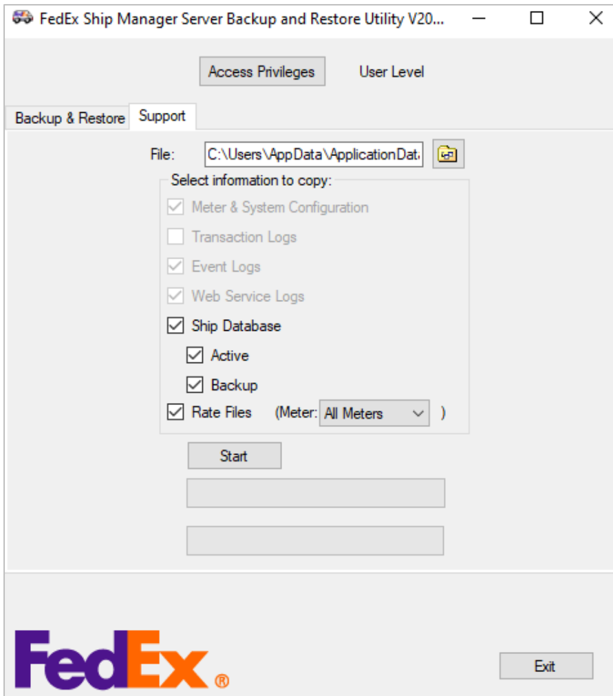
Figure 122: Support functionality
