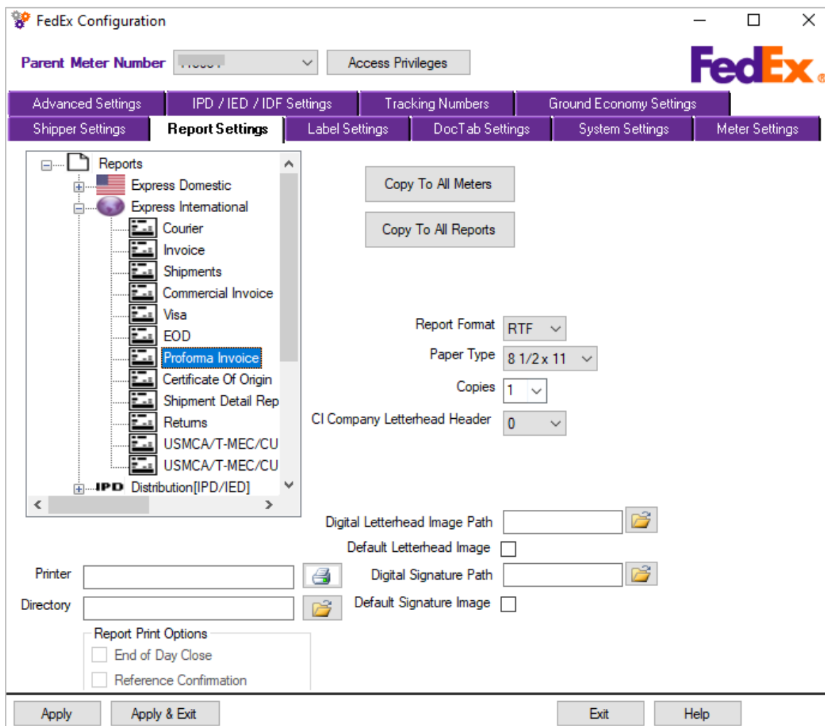
Figure 115: Reports Settings tab
