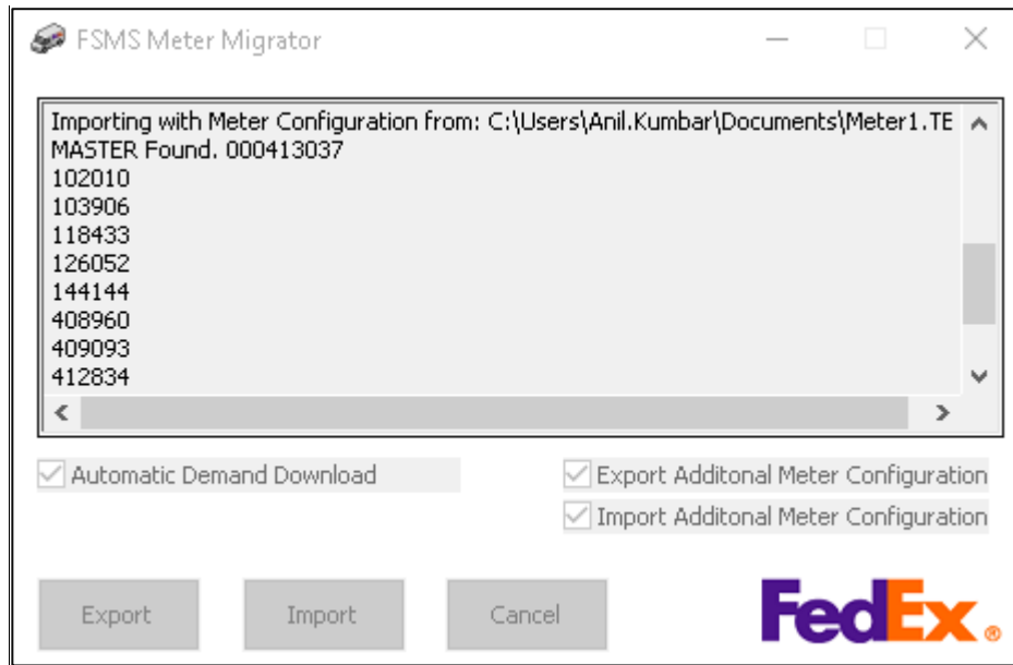
Figure 99: Import operation
