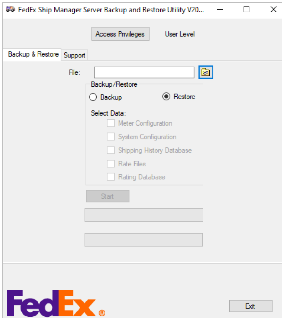
Figure 121: Restore functionality
