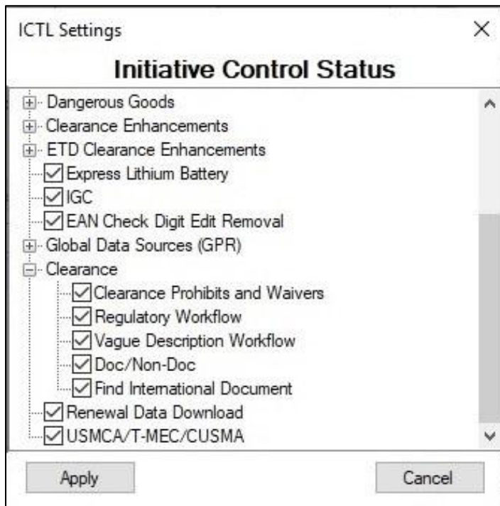
Figure 103: ICTL Settings with renamed branch Clearance
