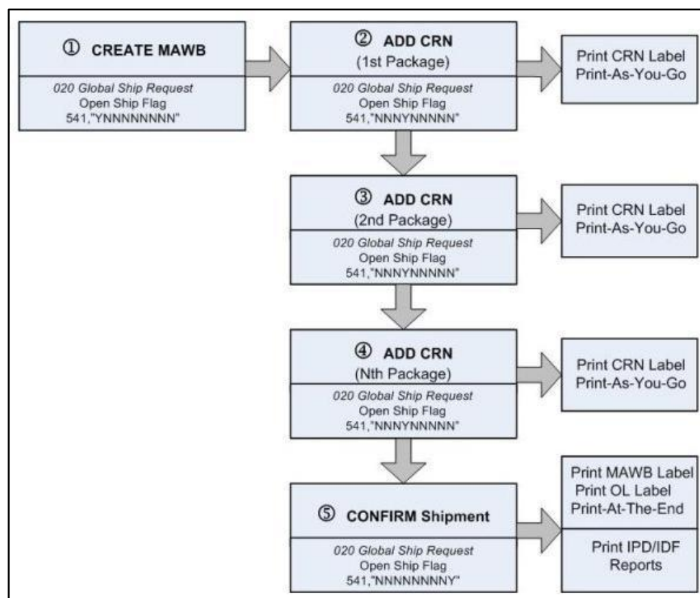
Figure 40: IPD/IDF/IED transaction workflow
