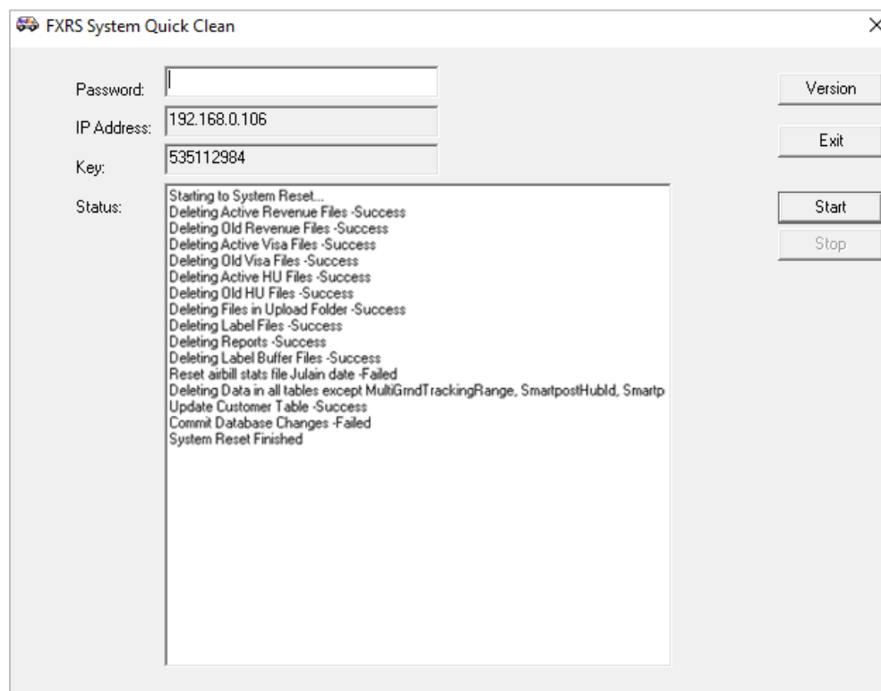
Figure 101: Quick Clean Process completion
