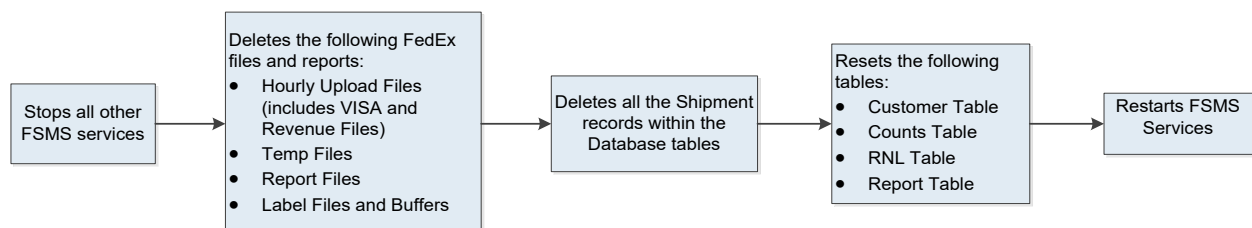
Figure 100: Quick Clean Utility functional flow
